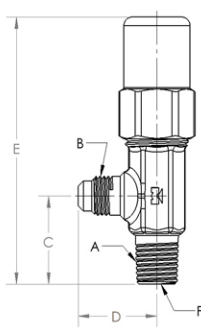
NPTFE Inlet to Flare
