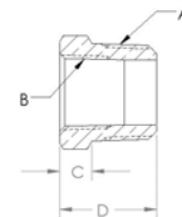
Bushing NPT to NPTFI
