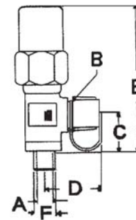
Solder to Flare
