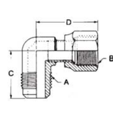
Ext FI to Int FI Swivel
