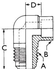
Half Union - Flare to Solder
