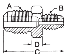
Reducing Unions - Fl to Fl
